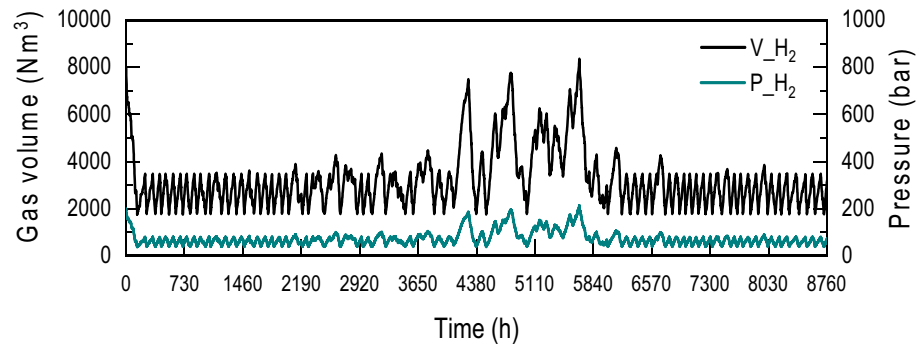
Fig. 13. Level of volume and pressure per hour of hydrogen storage of the optimal hybrid system over the year.
